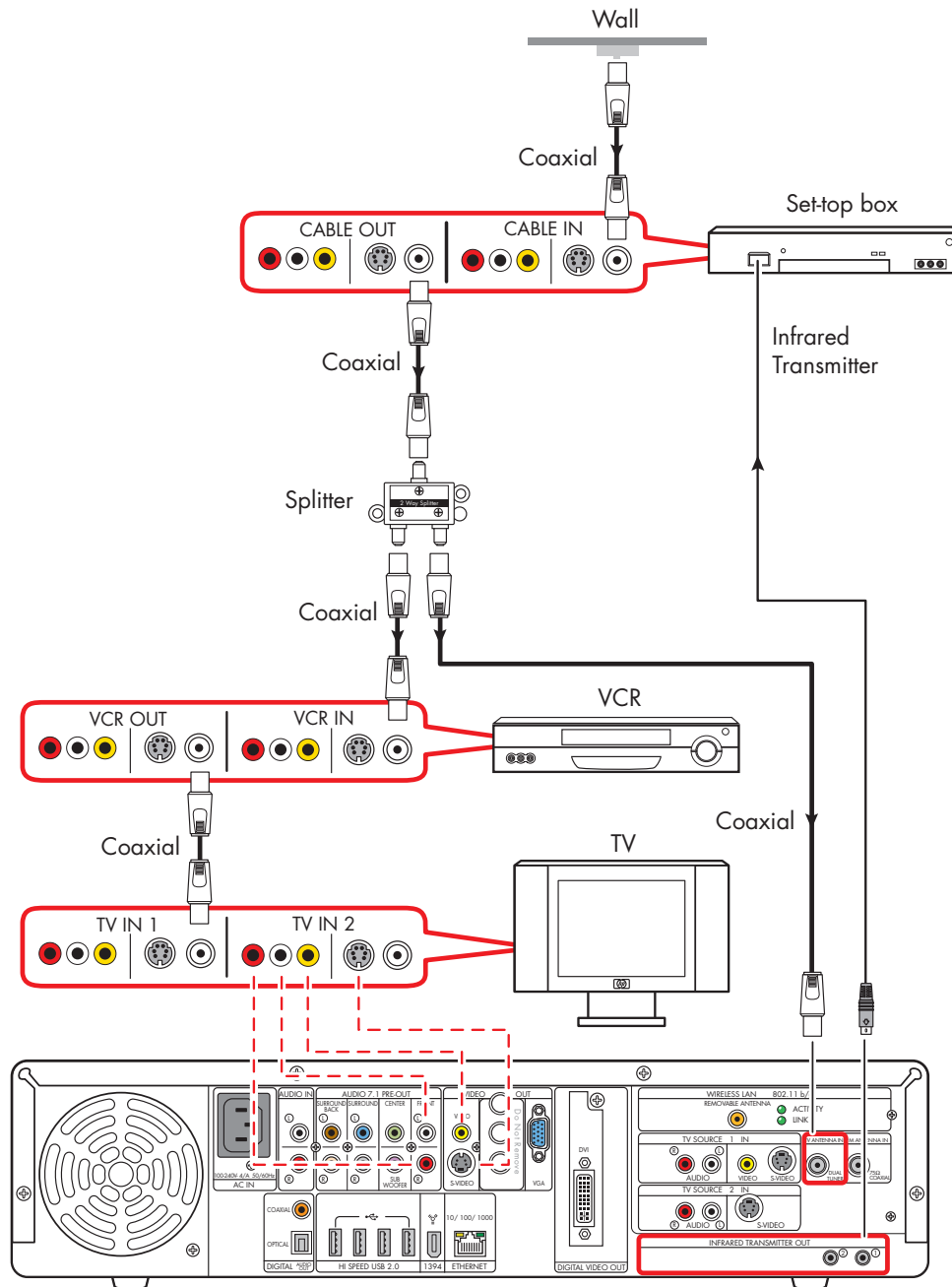
Wall to set-top box VCR to TV using coaxial cable (add with a splitter)
